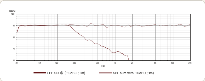
LFE Frequency Response
