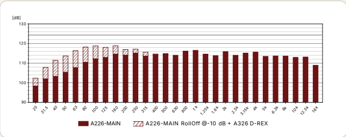
Max Continuous SPL
