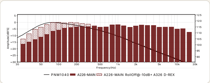
PN M 1040 Spectrum vs Max Continuous SPL
