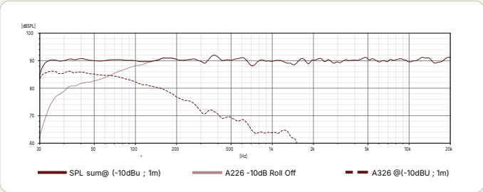
Combined Frequency Response
